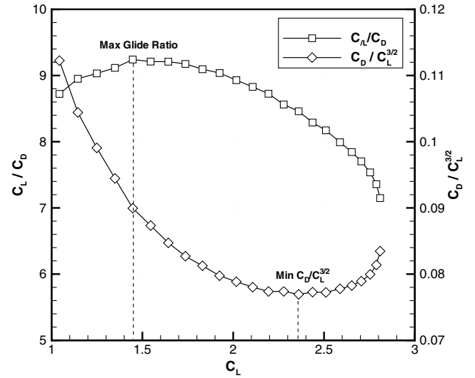
Fig. 4 Glide ratio and descent factor f_d [Eq. (8)] of the Alvast/A-310 scale model wing.
