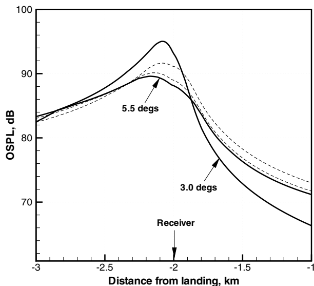
Fig. 21 Calculated OSPL of aircraft model at FAR landing point; W = 110 tons.
